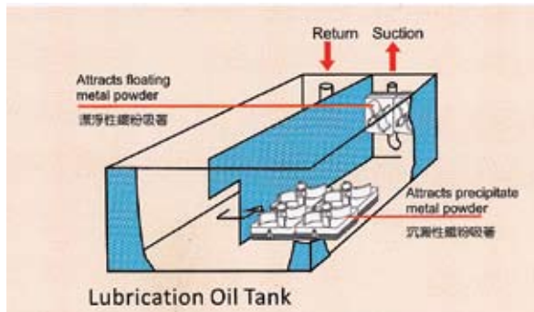
Lubrication Oil Tank
